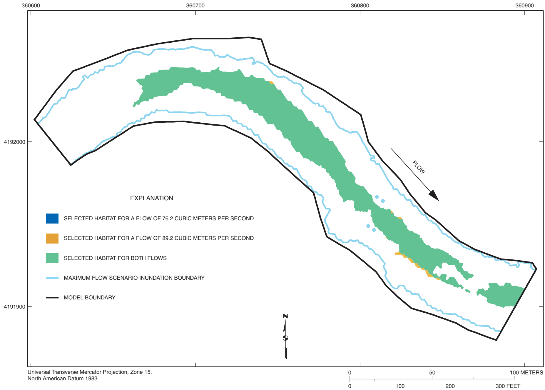
Figure 1-24. Selected habitat area distribution for habitat category 7 (paddlefish) at flows of 76.2 and 89.2 cubic meters per second at Marmaton River site M1.
